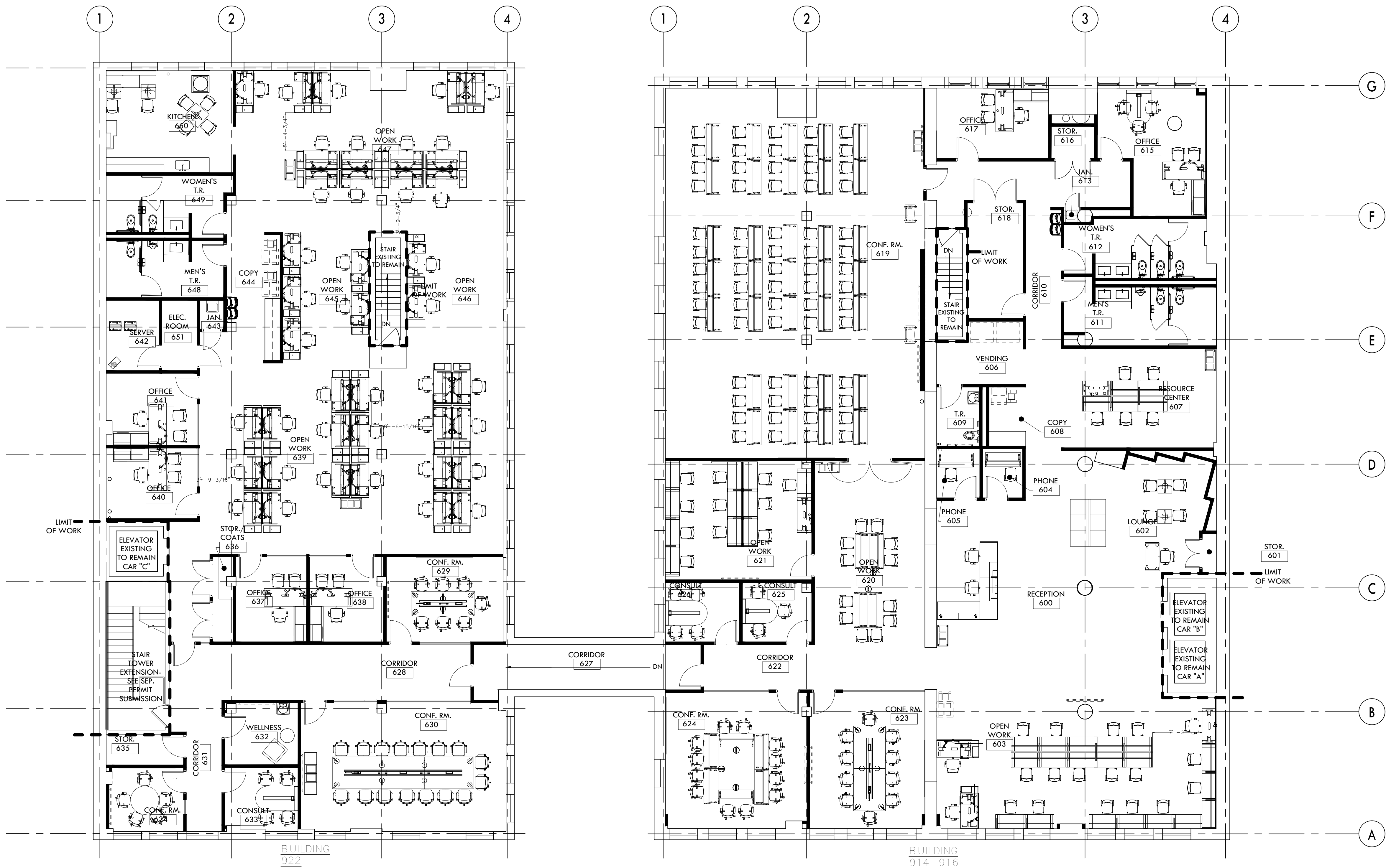
1: FURNITURE PLAN
